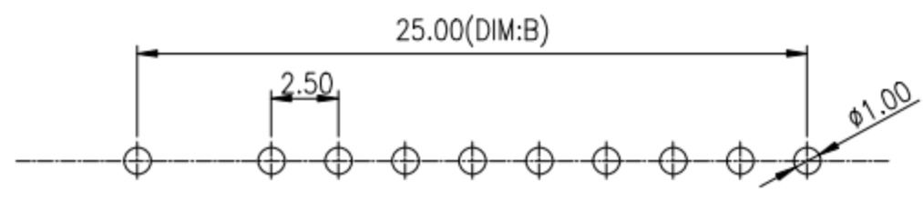
Recommended P.C.B Layout Layout Tolerance=+/-0.05mm
